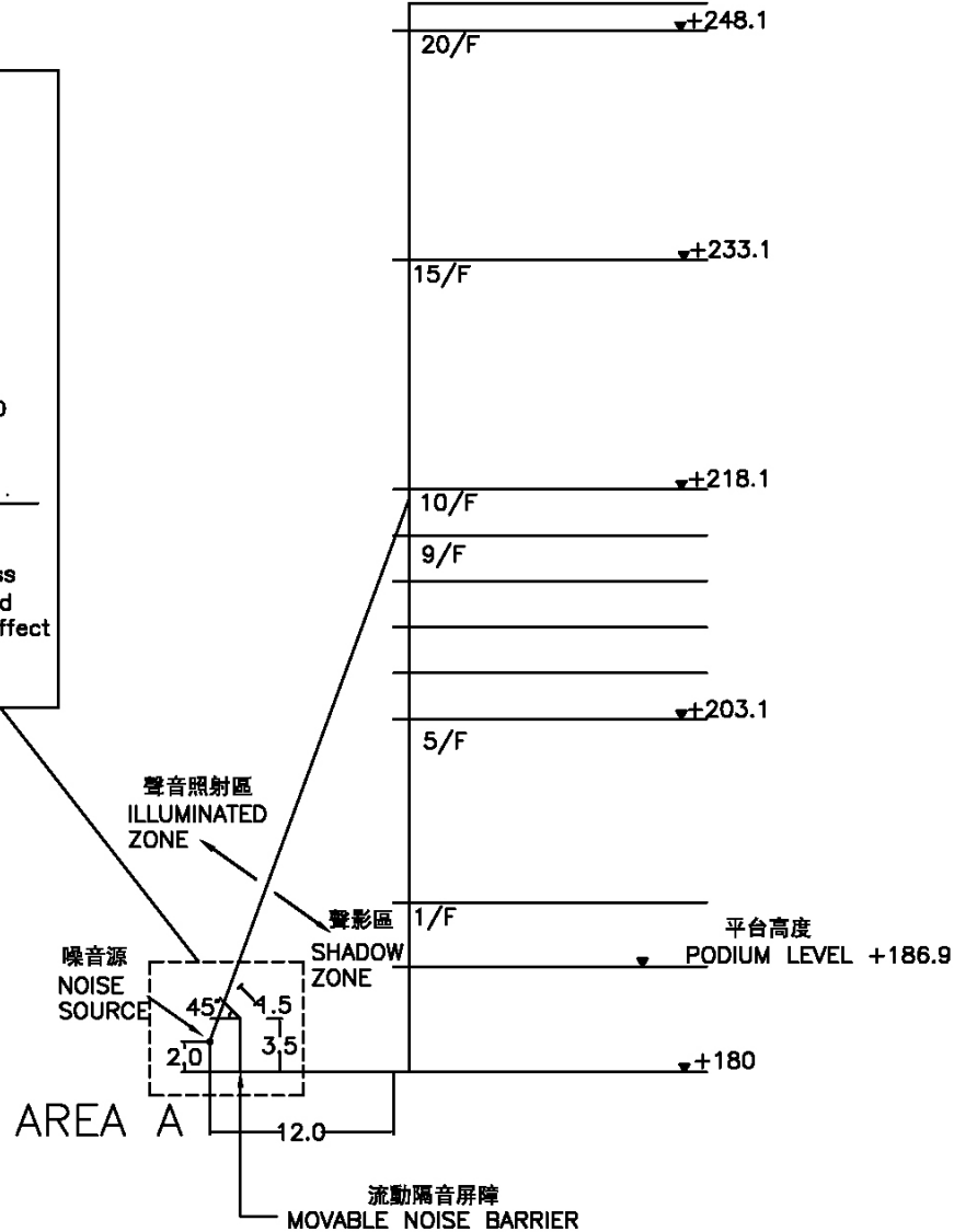
Figure 8 - 1 : Typical Section of Movable Noise Barrier (for part II of the project) 圖 8 - 1 : 流動隔音屏障的切面圖 (適用於工程項目第 II 部份)
